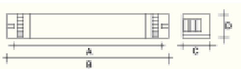
FIG. A A = 220 mm B = 226 mm C = 30 mm D = 23 mm FIG. B A = 350 mm B = 356 mm C = 30 mm D = 23 mm
